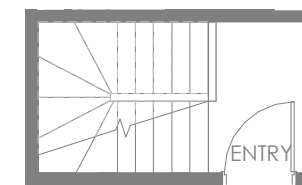
UPPER FLOOR
